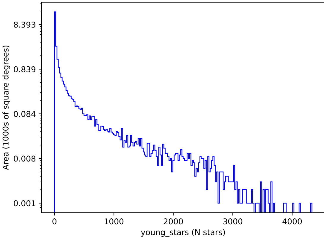
too_combined_s1.5_v3.4_10yrs : young_stars
