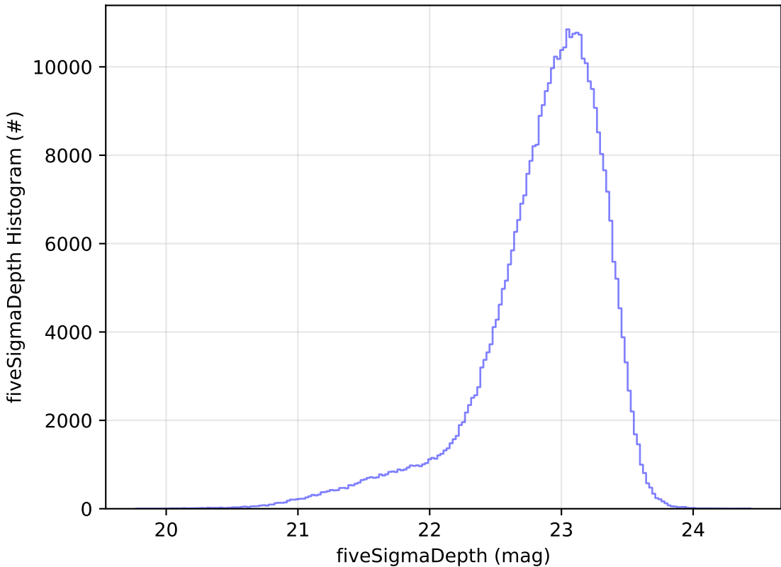
too_combined_s1.5_v3.4_10yrs z: fiveSigmaDepth Histogram
