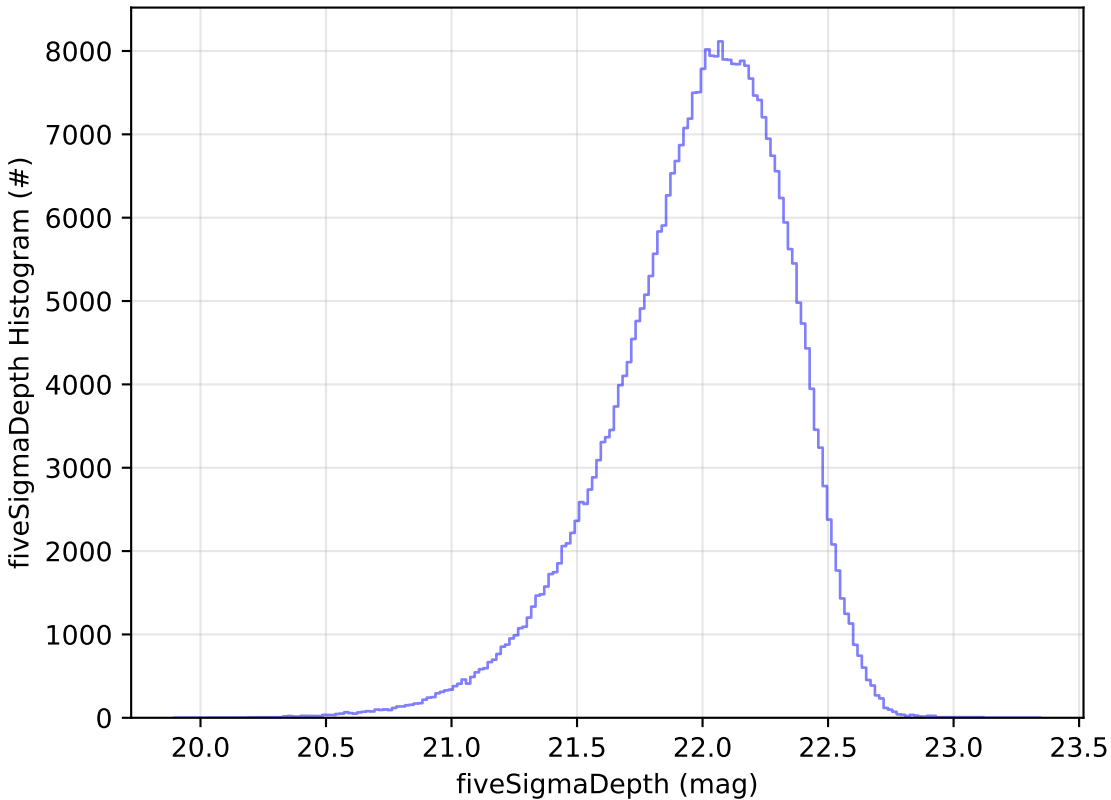
too_combined_s1.5_v3.4_10yrs y: fiveSigmaDepth Histogram
