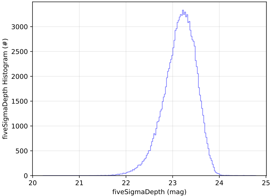
too_combined_s1.5_v3.4_10yrs u: fiveSigmaDepth Histogram
