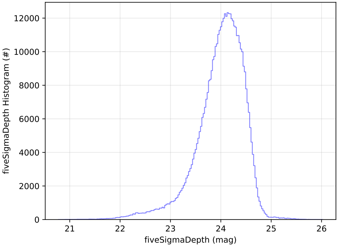
too_combined_s1.5_v3.4_10yrs r: fiveSigmaDepth Histogram
