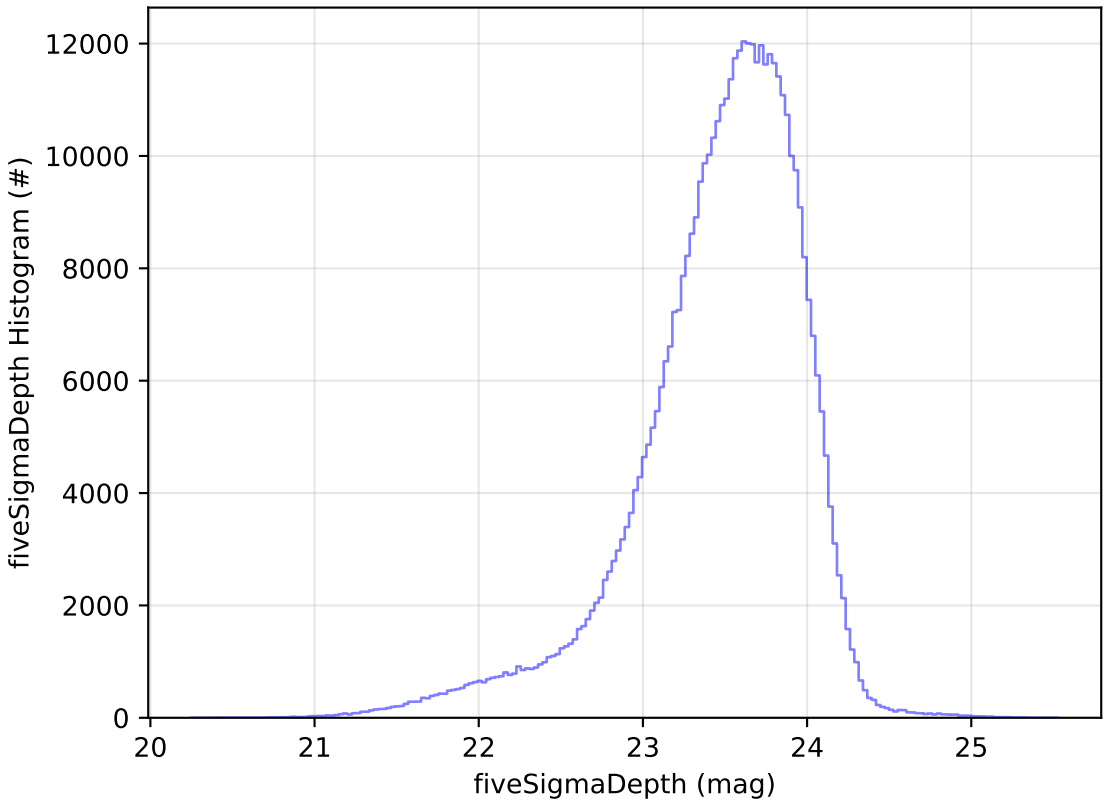
too_combined_s1.5_v3.4_10yrs i: fiveSigmaDepth Histogram
