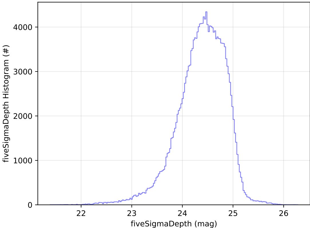
too_combined_s1.5_v3.4_10yrs g: fiveSigmaDepth Histogram
