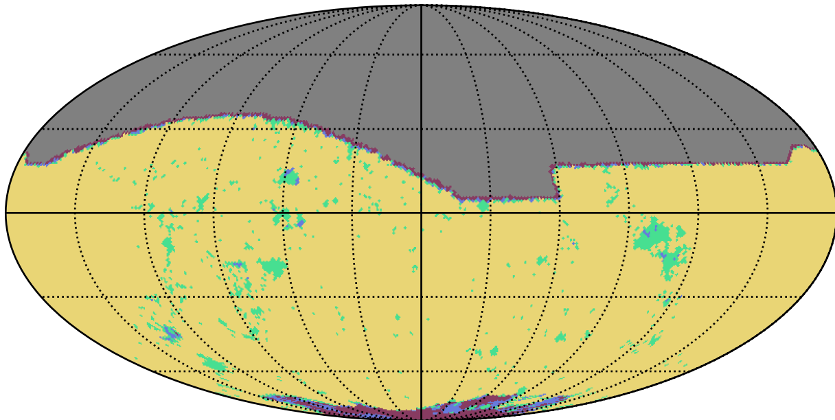
too_combined_s1.5_v3.4_10yrs i band: YearCoverage night
