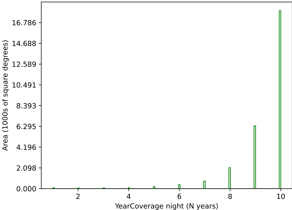
too_combined_s1.5_v3.4_10yrs g band: YearCoverage night
