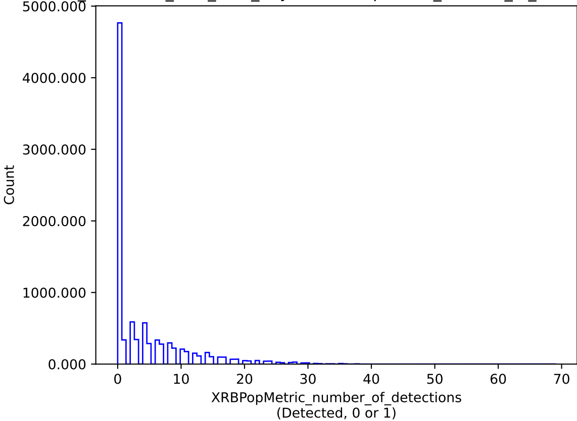
too_combined_s1.5_v3.4_10yrs : XRBPopMetric_number_of_detections
