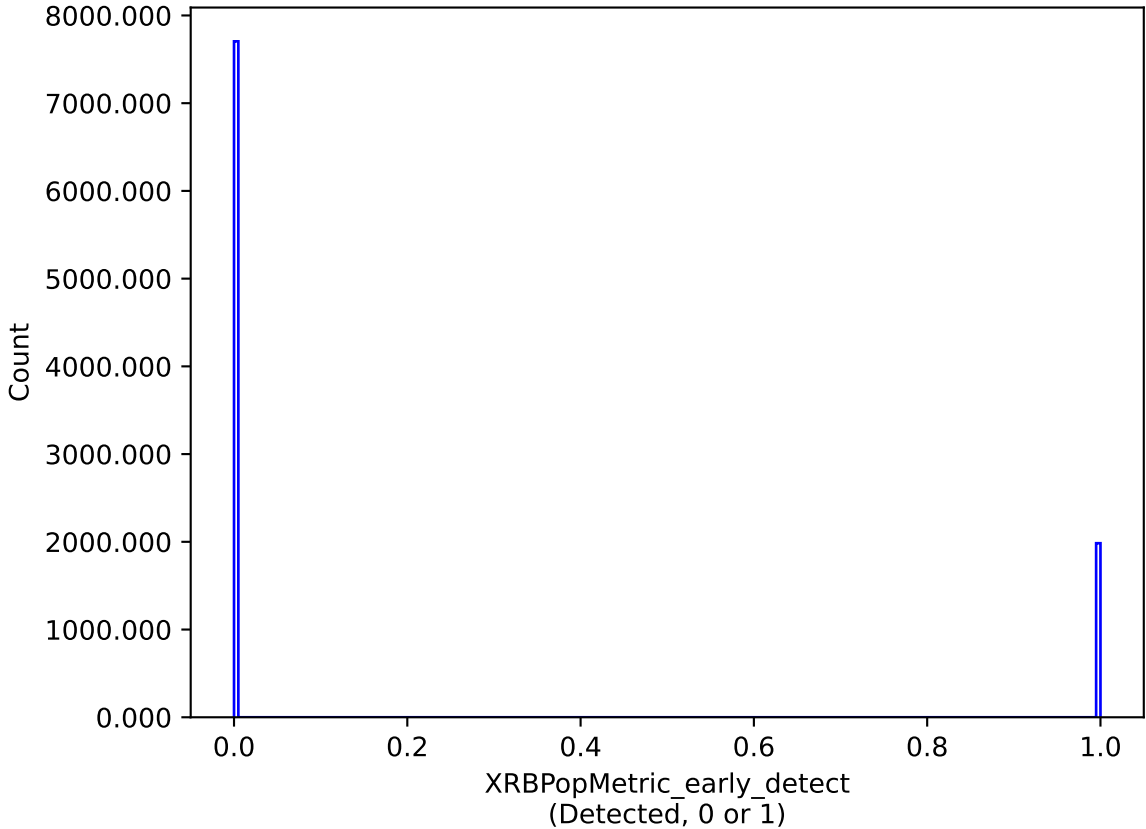
too_combined_s1.5_v3.4_10yrs : XRBPopMetric_early_detect
