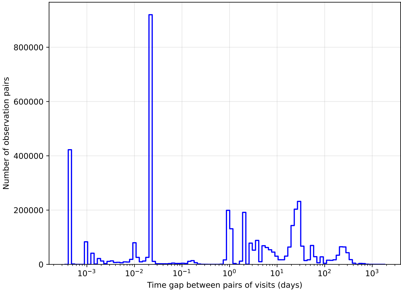
too_combined_s1.5_v3.4_10yrs y band: Tgaps observationStartMJD
