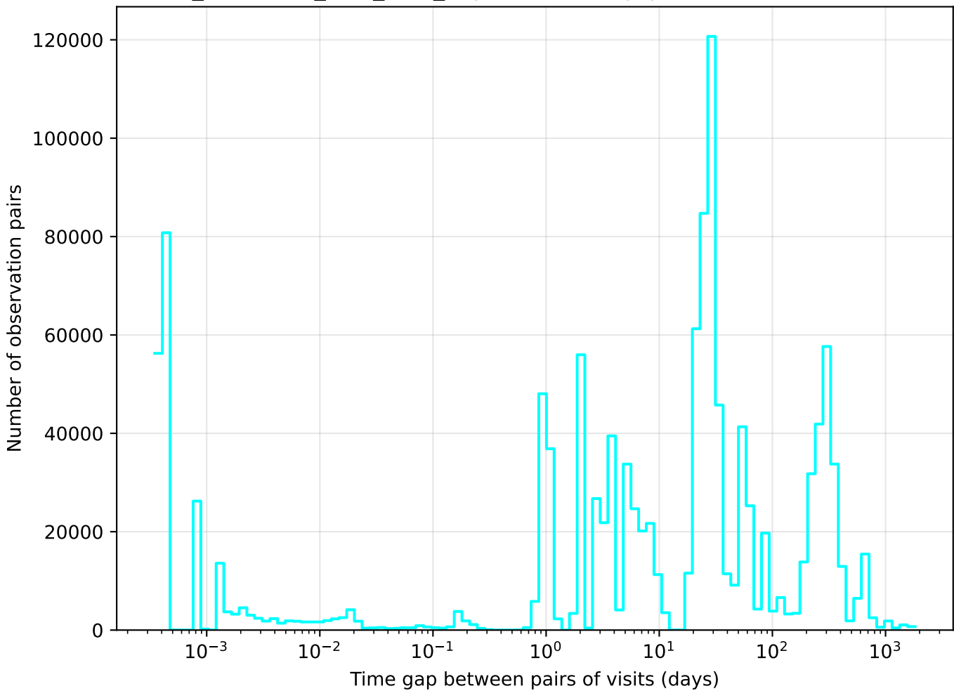
too_combined_s1.5_v3.4_10yrs u band: Tgaps observationStartMJD
