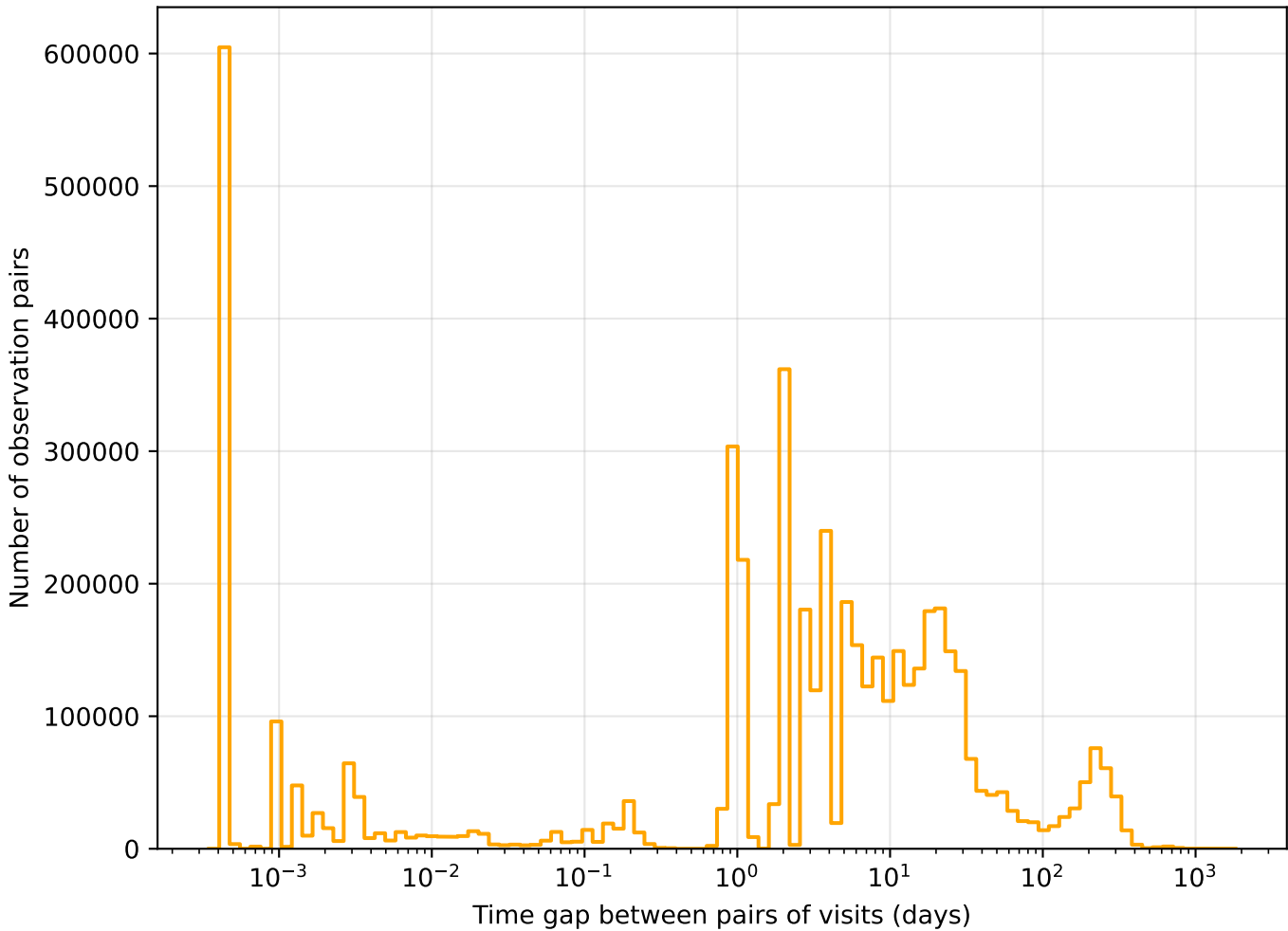
too_combined_s1.5_v3.4_10yrs r band: Tgaps observationStartMJD
