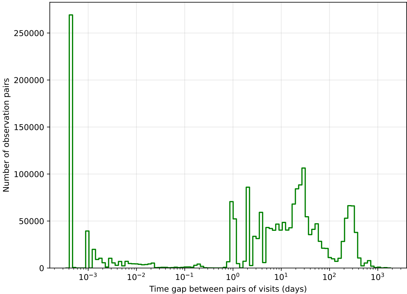
too_combined_s1.5_v3.4_10yrs g band: Tgaps observationStartMJD
