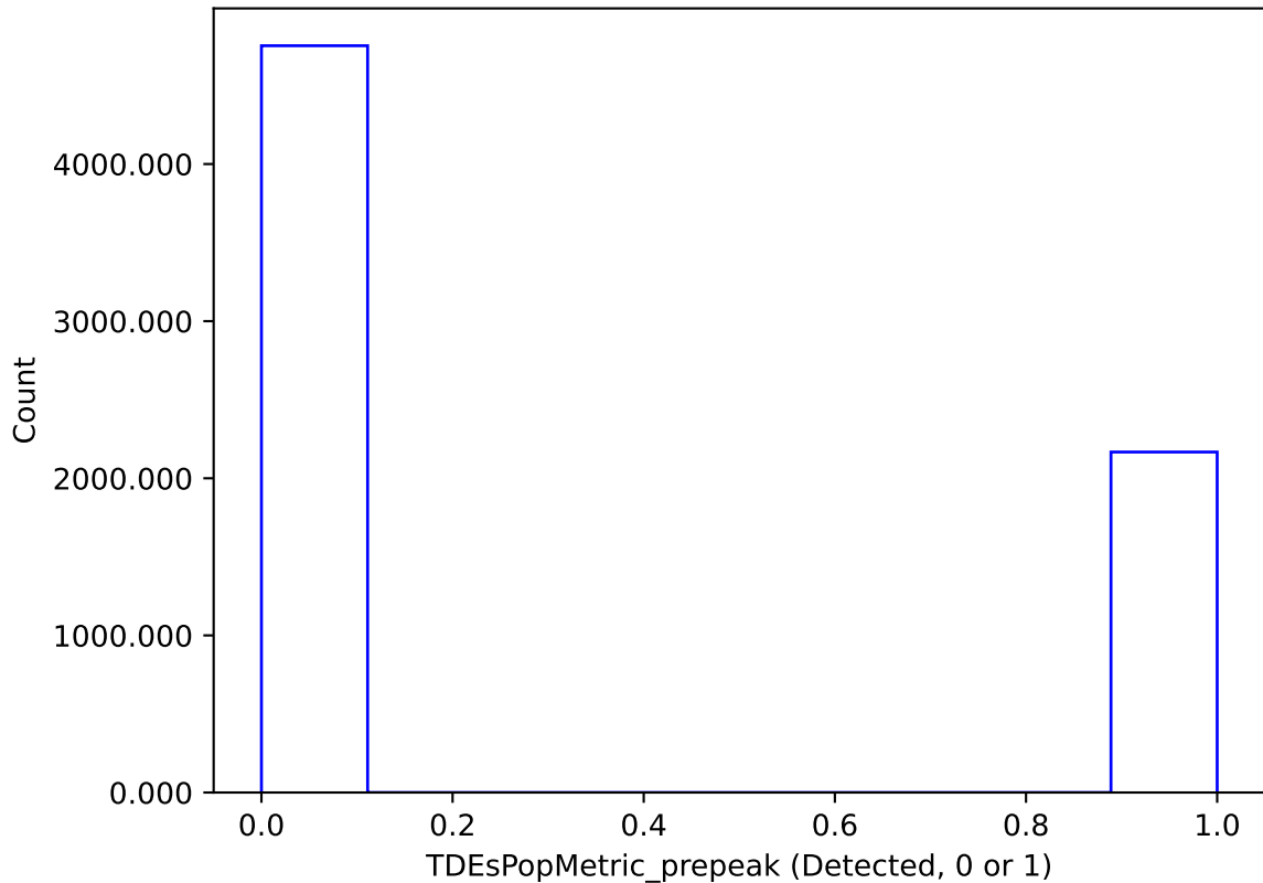
too_combined_s1.5_v3.4_10yrs : TDEsPopMetric_prepeak
