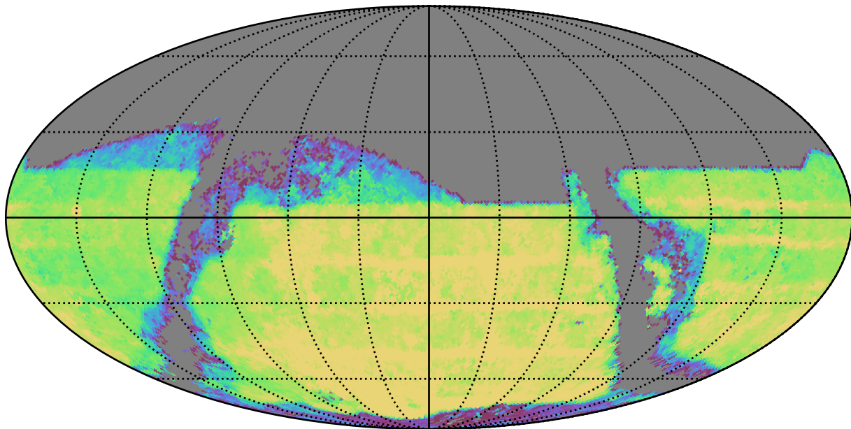
too_combined_s1.5_v3.4_10yrs : TDC_season
