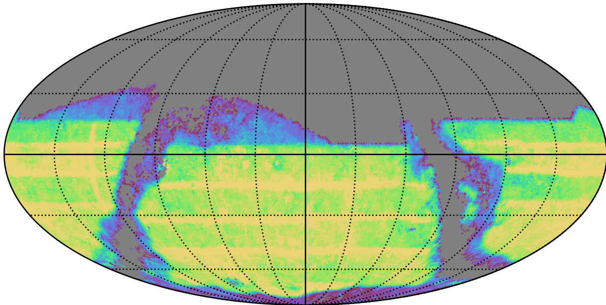
too_combined_s1.5_v3.4_10yrs : TDC_rate
