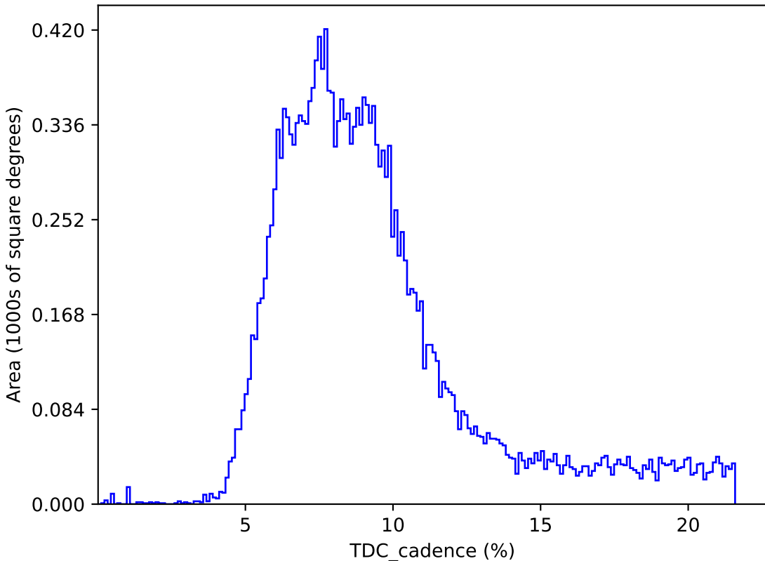
too_combined_s1.5_v3.4_10yrs : TDC_cadence
