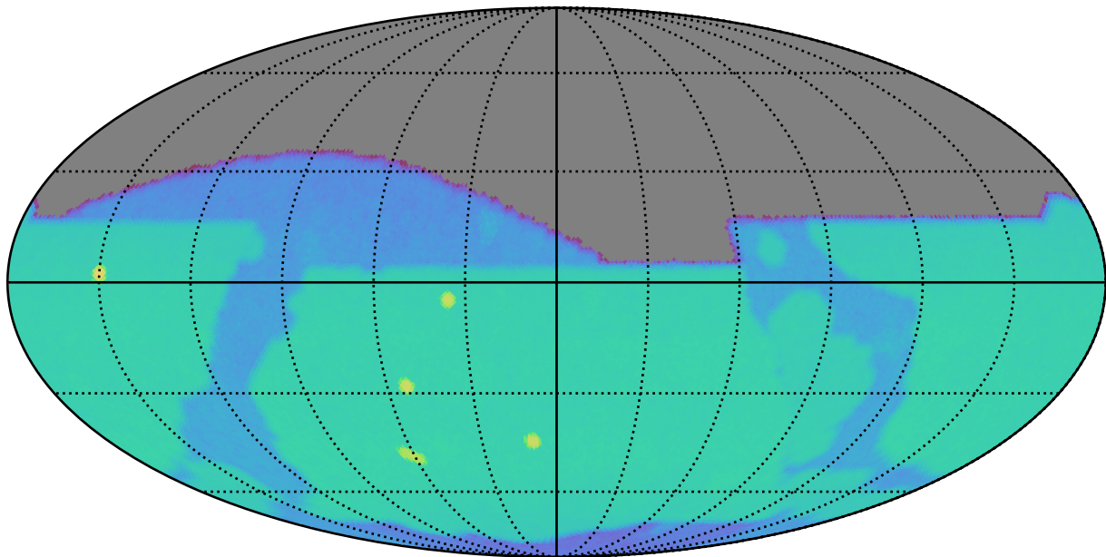
too_combined_s1.5_v3.4_10yrs z: SurfaceBrightLimit
