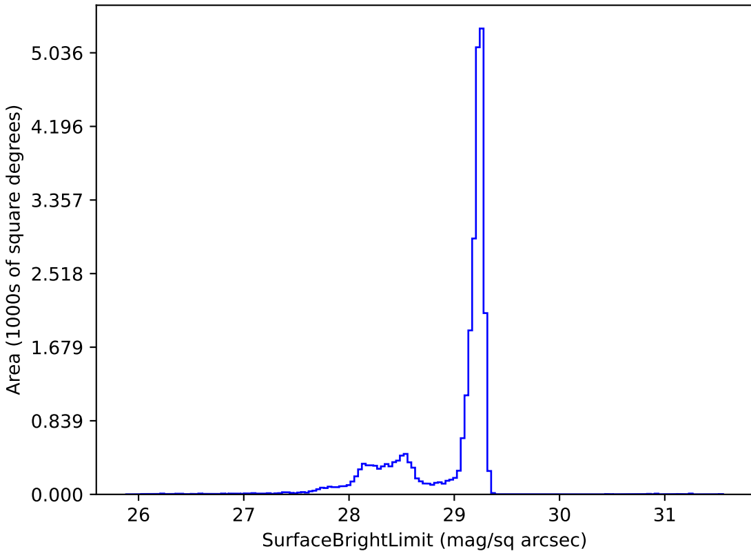
too_combined_s1.5_v3.4_10yrs z: SurfaceBrightLimit
