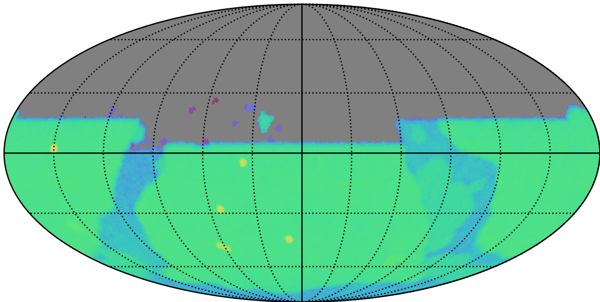
too_combined_s1.5_v3.4_10yrs u: SurfaceBrightLimit
