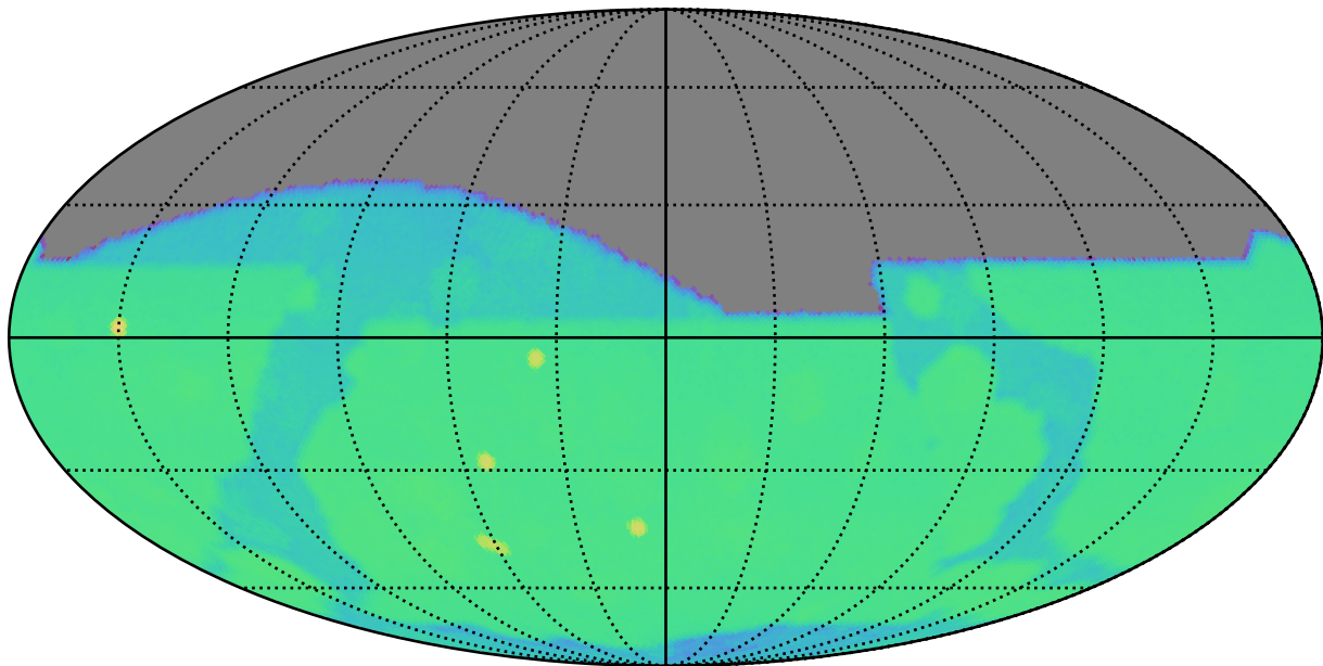
too_combined_s1.5_v3.4_10yrs r: SurfaceBrightLimit
