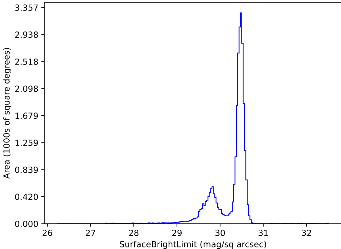
too_combined_s1.5_v3.4_10yrs r: SurfaceBrightLimit
