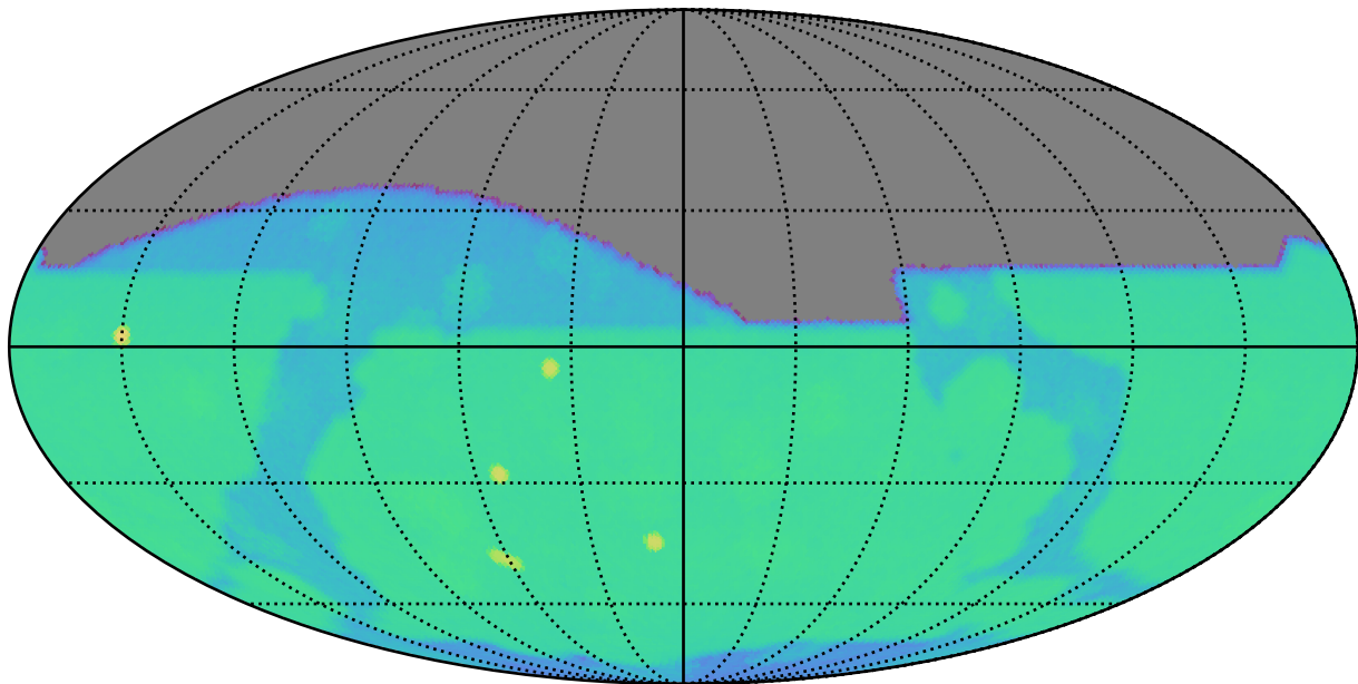
too_combined_s1.5_v3.4_10yrs i: SurfaceBrightLimit
