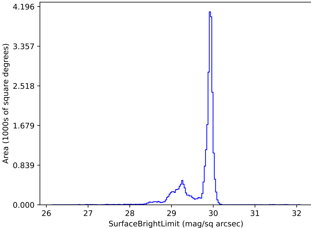
too_combined_s1.5_v3.4_10yrs i: SurfaceBrightLimit
