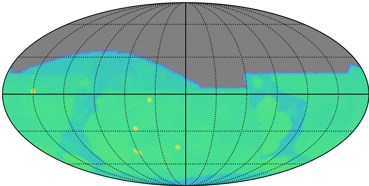
too_combined_s1.5_v3.4_10yrs g: SurfaceBrightLimit
