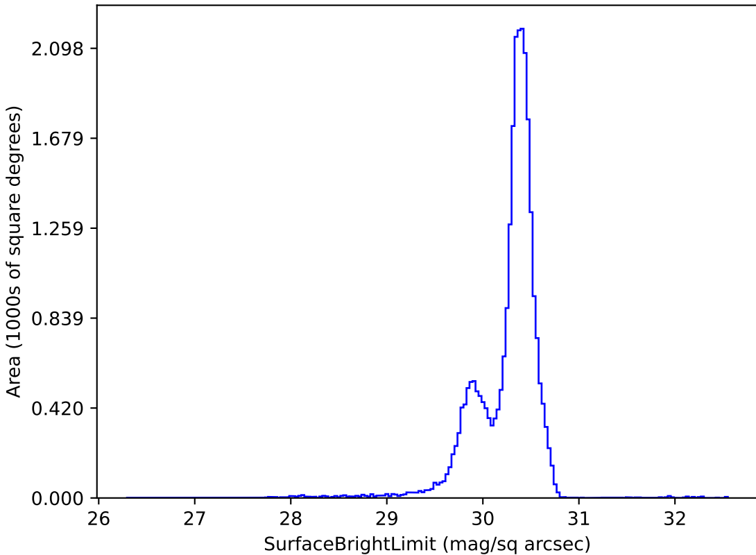
too_combined_s1.5_v3.4_10yrs g: SurfaceBrightLimit
