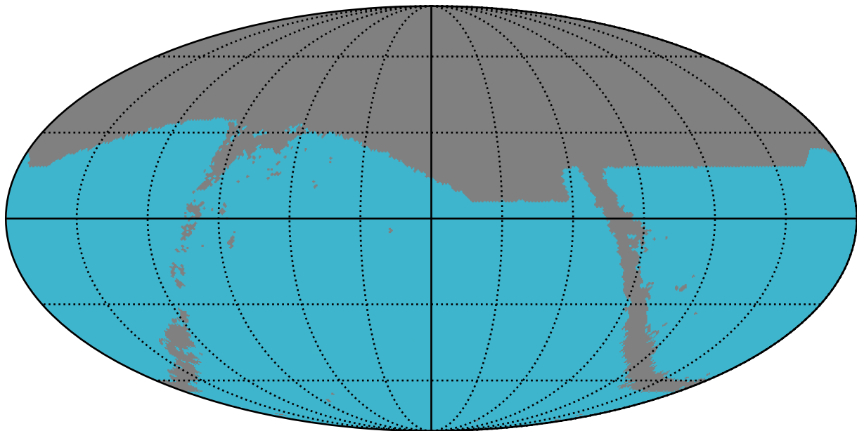
too_combined_s1.5_v3.4_10yrs : SNSLMetric
