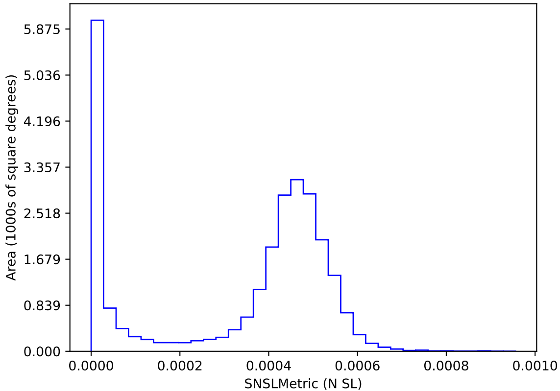
too_combined_s1.5_v3.4_10yrs : SNSLMetric
