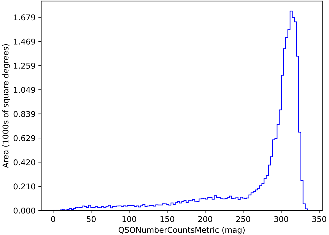
too_combined_s1.5_v3.4_10yrs u band and non-DD: QSONumberCountsMetric
