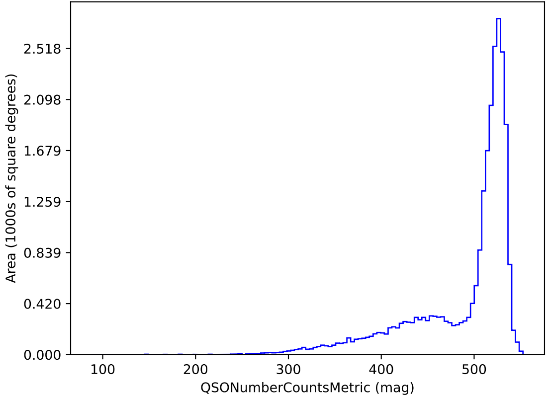
too_combined_s1.5_v3.4_10yrs r band and non-DD: QSONumberCountsMetric
