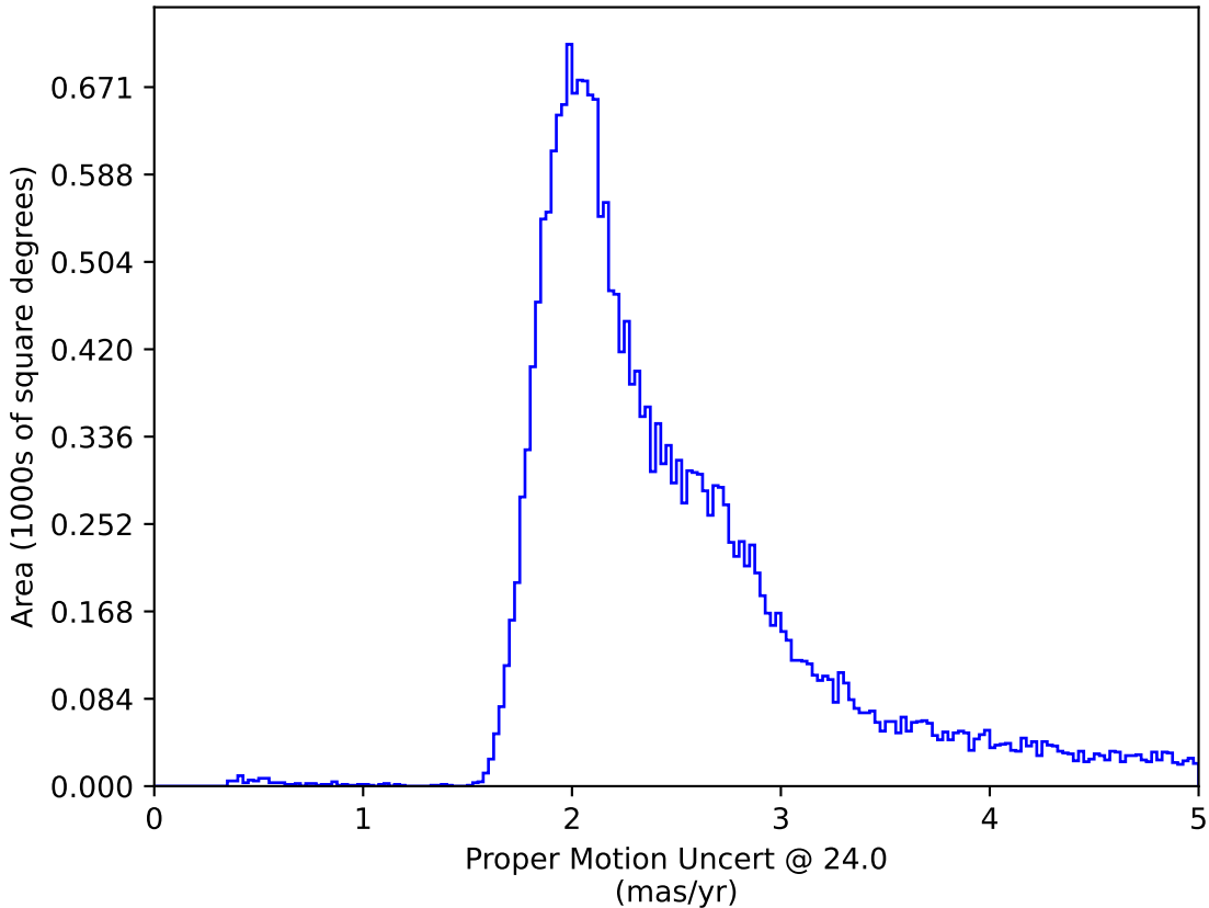
too_combined_s1.5_v3.4_10yrs : Proper Motion Uncert @ 24.0
