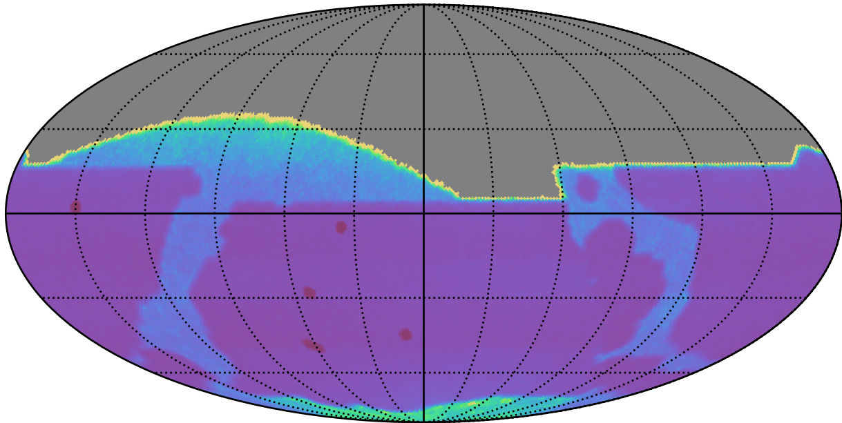
too_combined_s1.5_v3.4_10yrs : Proper Motion Uncert @ 20.5
