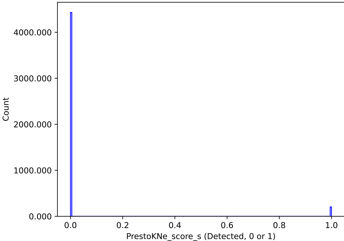
too_combined_s1.5_v3.4_10yrs : PrestoKNe_score_s
