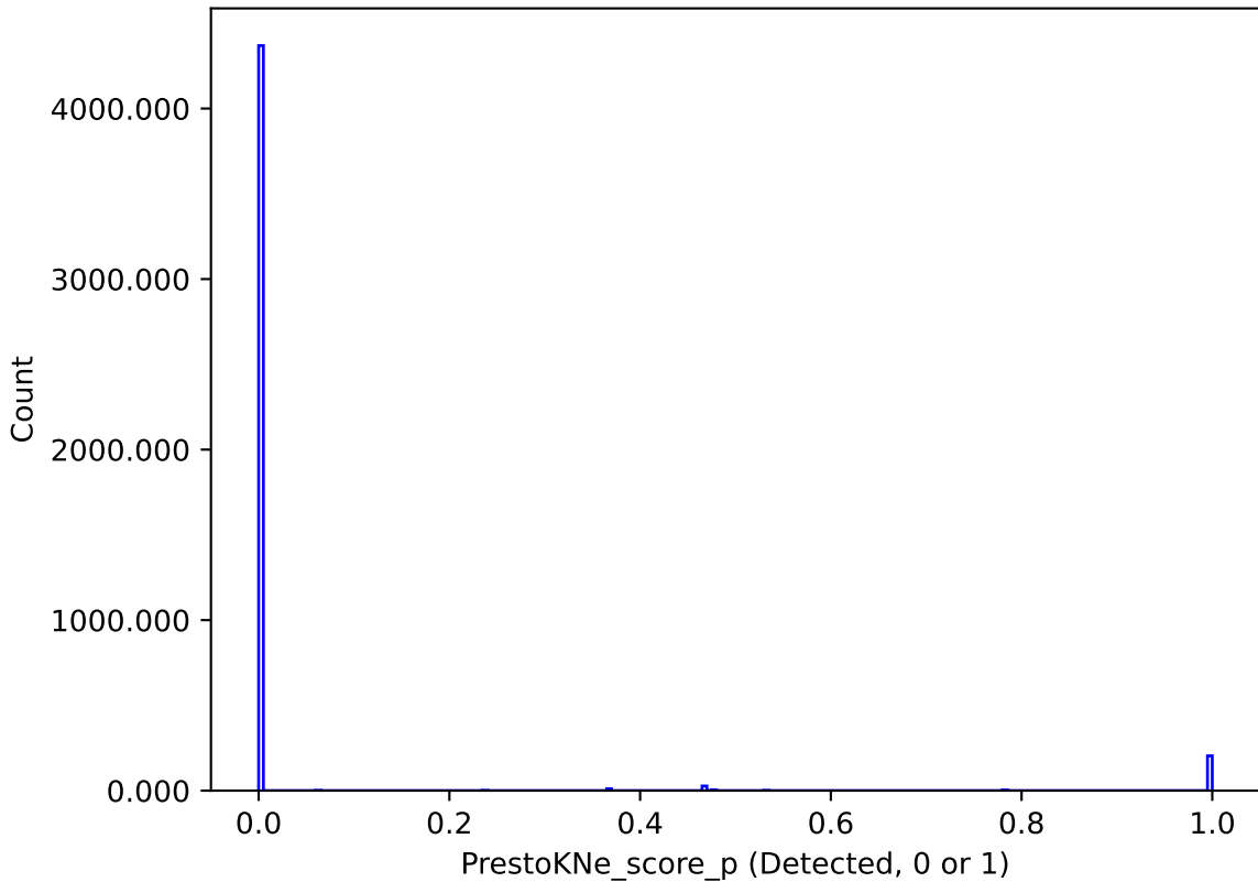
too_combined_s1.5_v3.4_10yrs : PrestoKNe_score_p
