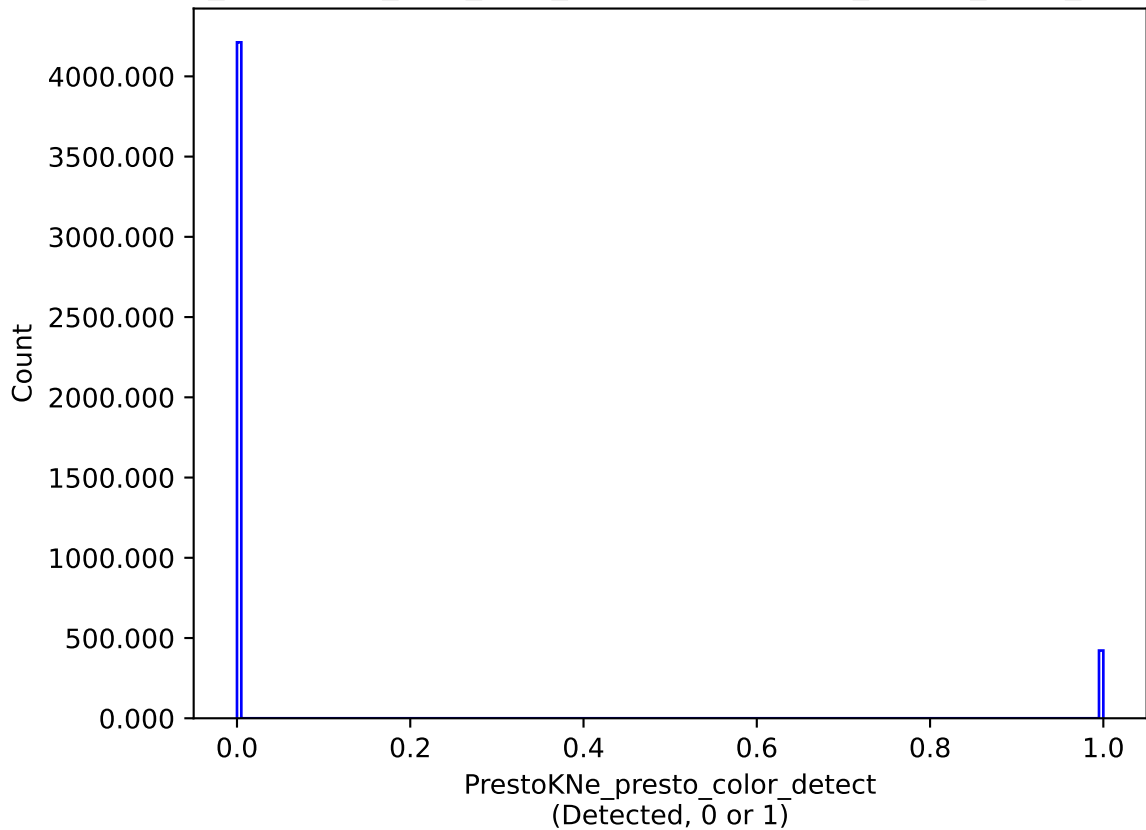
too_combined_s1.5_v3.4_10yrs : PrestoKNe_presto_color_detect
