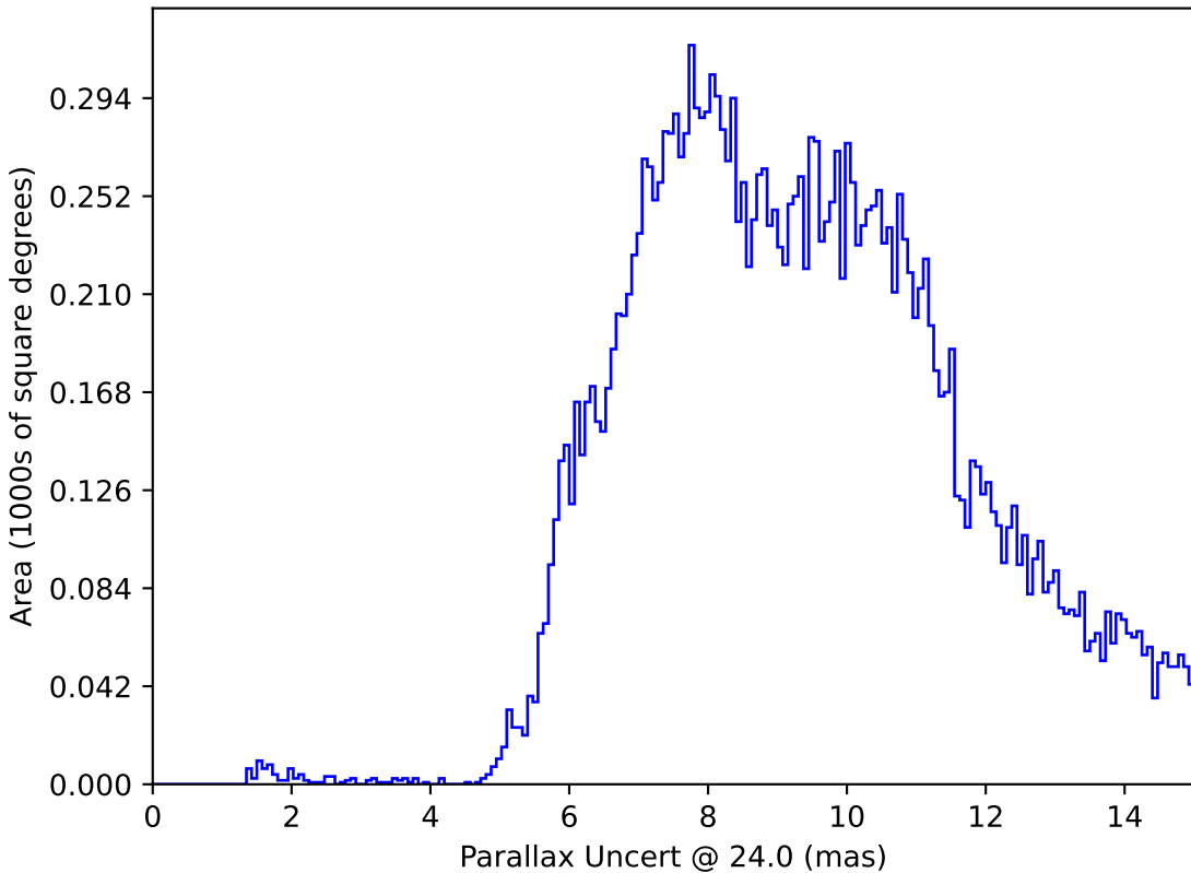
too_combined_s1.5_v3.4_10yrs : Parallax Uncert @ 24.0
