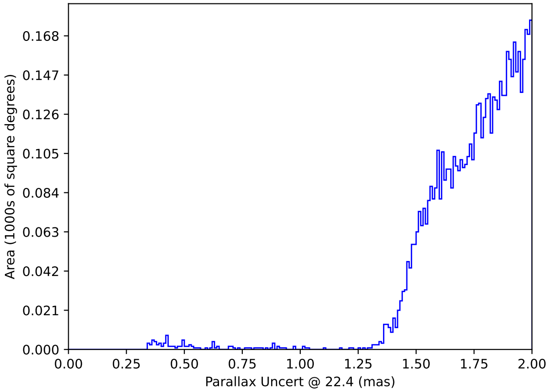
too_combined_s1.5_v3.4_10yrs : Parallax Uncert @ 22.4
