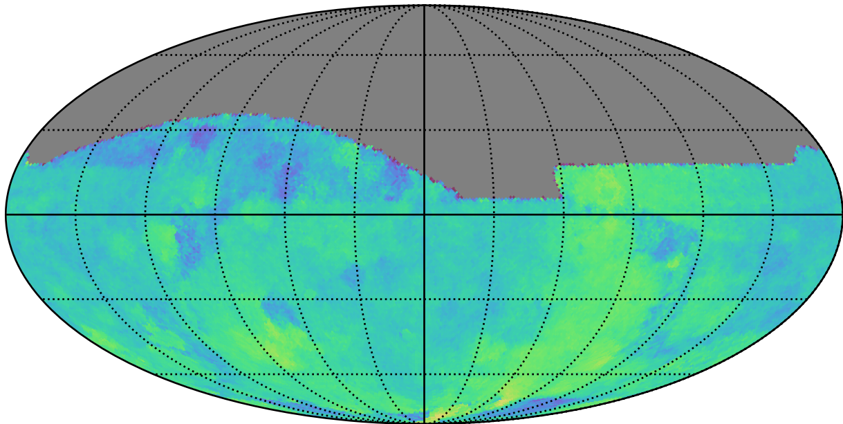
too_combined_s1.5_v3.4_10yrs : Parallax Coverage @ 24.0
