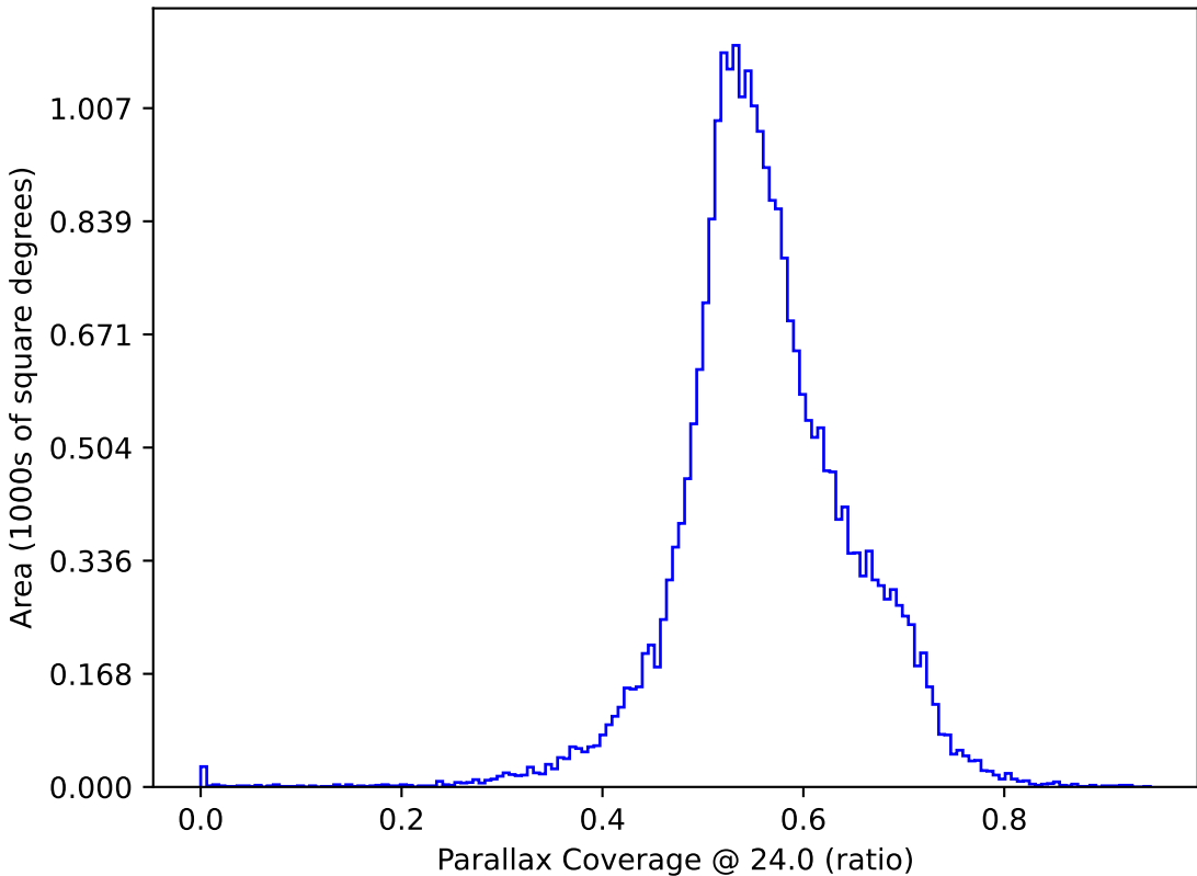
too_combined_s1.5_v3.4_10yrs : Parallax Coverage @ 24.0
