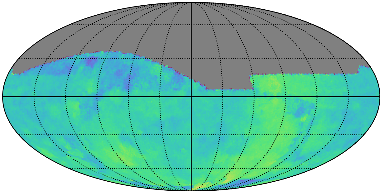
too_combined_s1.5_v3.4_10yrs : Parallax Coverage @ 22.4
