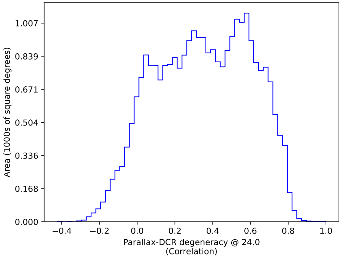
too_combined_s1.5_v3.4_10yrs : Parallax-DCR degeneracy @ 24.0
