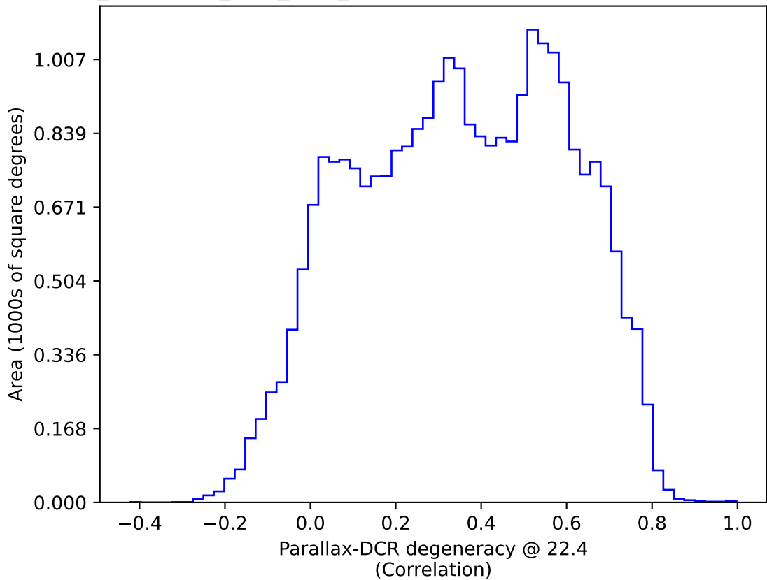
too_combined_s1.5_v3.4_10yrs : Parallax-DCR degeneracy @ 22.4
