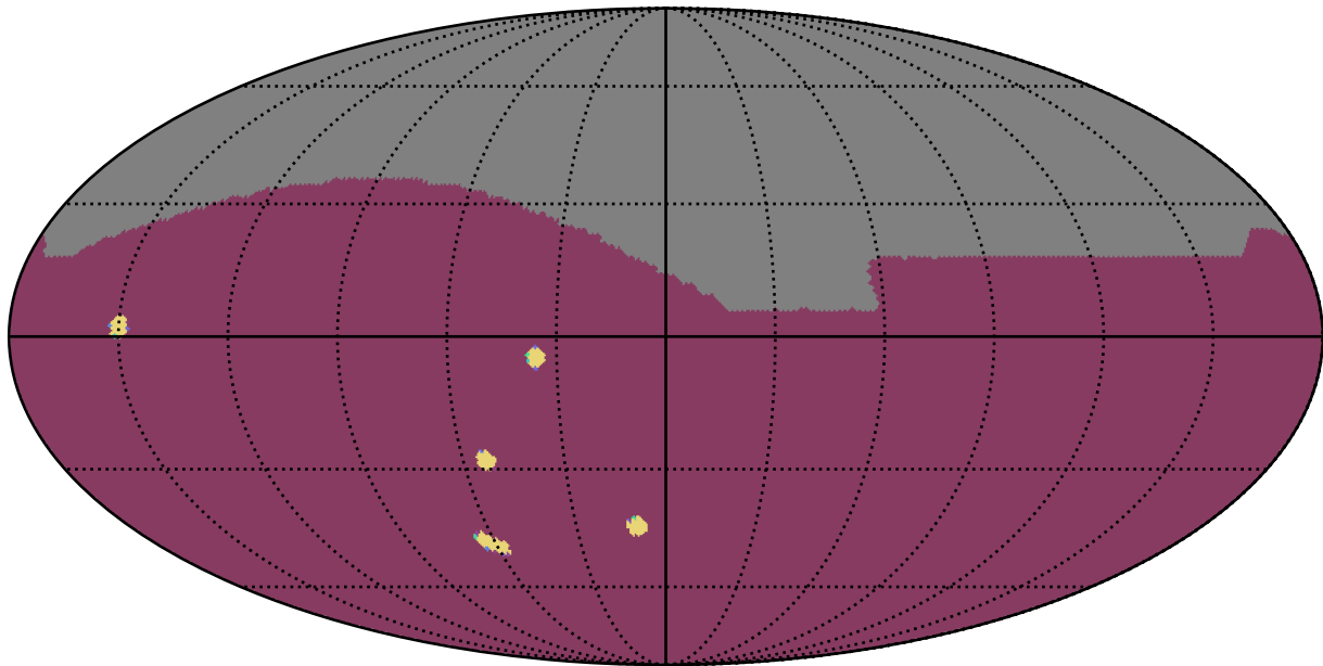
too_combined_s1.5_v3.4_10yrs : NumberOfQuickRevisits
