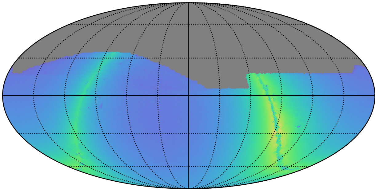
too_combined_s1.5_v3.4_10yrs z: Nstars_no_crowding
