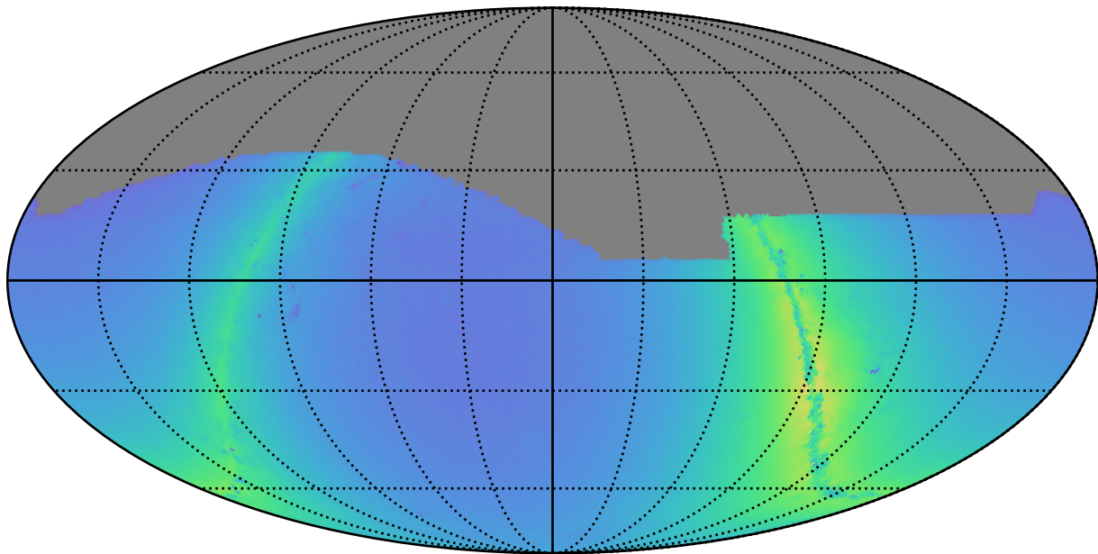
too_combined_s1.5_v3.4_10yrs r: Nstars_no_crowding
