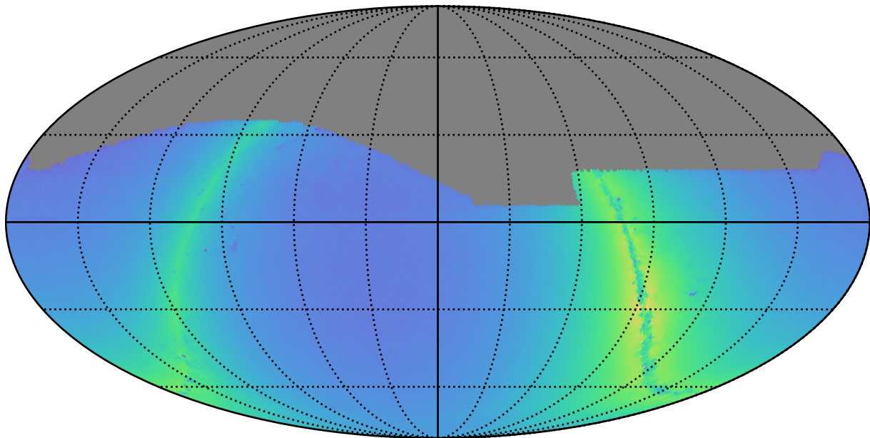
too_combined_s1.5_v3.4_10yrs i: Nstars_no_crowding
