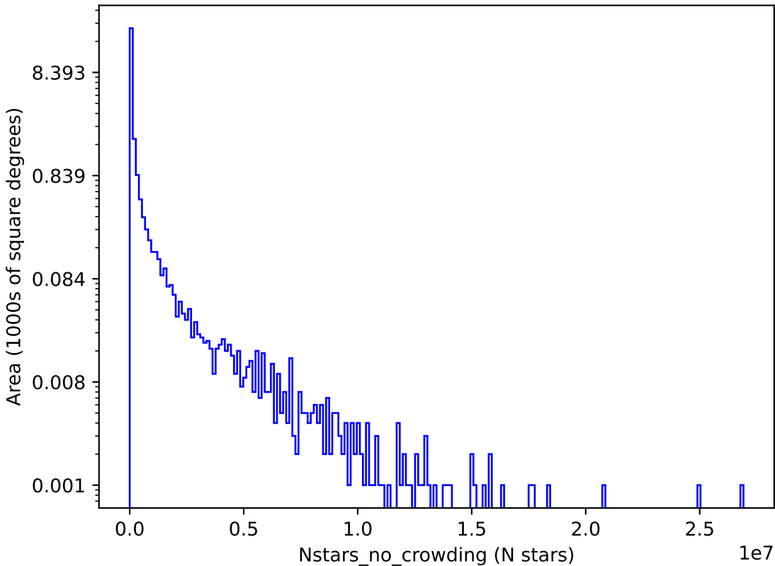
too_combined_s1.5_v3.4_10yrs i: Nstars_no_crowding
