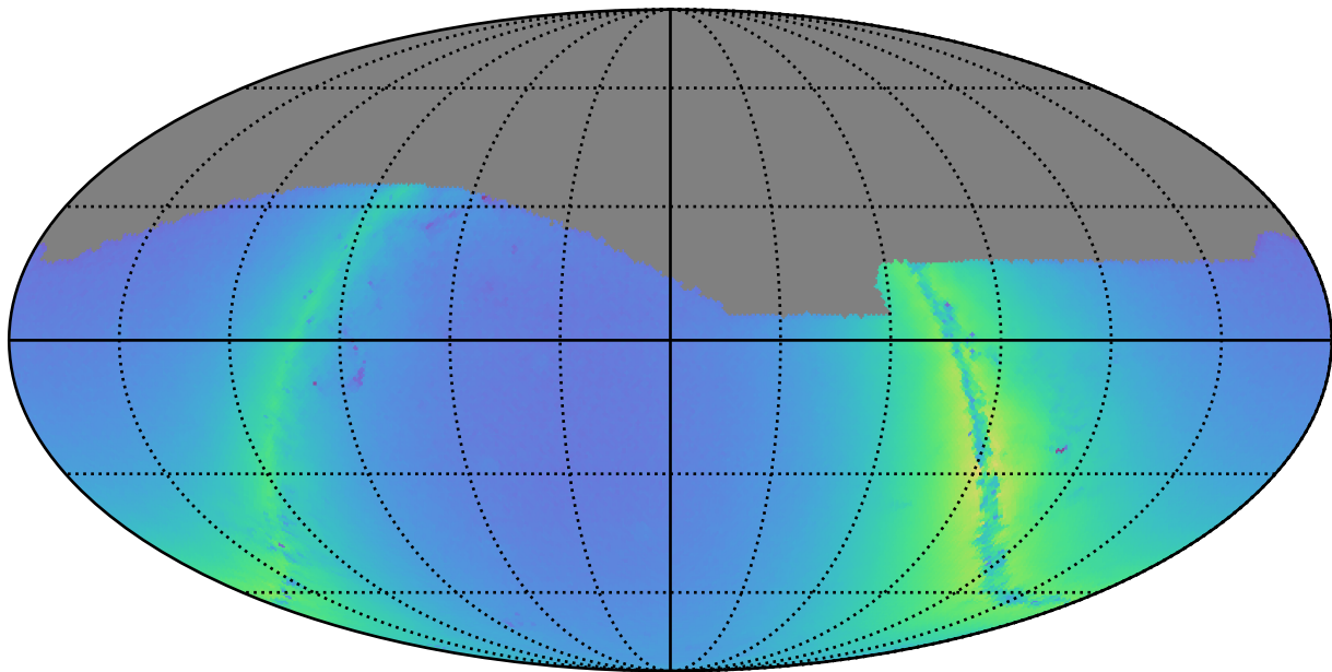
too_combined_s1.5_v3.4_10yrs g: Nstars_no_crowding
